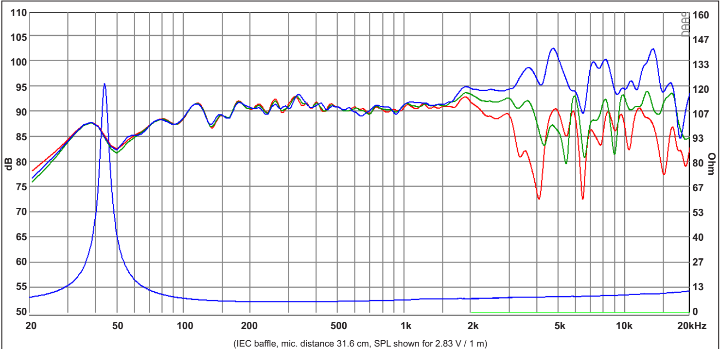
Response Curve : — (Blue) : on axis — (Green) : 30° off-axis — ( Red ) : 60° off-axis
